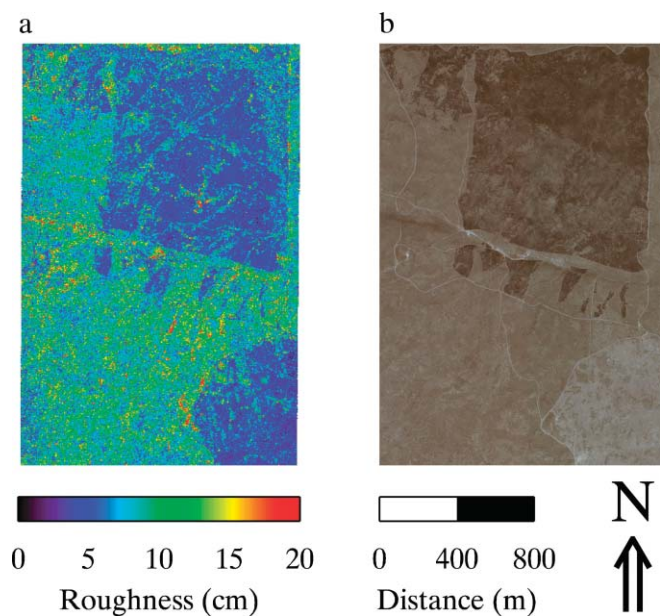
Figure 2. a, Map of calculated surface roughness after fire in Idaho, and b, QuickBird image of the same area. Reprinted from Streutker, D. and N. Glenn. 2006. LiDAR measurement of sagebrush steppe vegetation heights. Remote Sensing of Environment 102:135–145. Copyright 2006, reprinted with permission from Elsevier.
